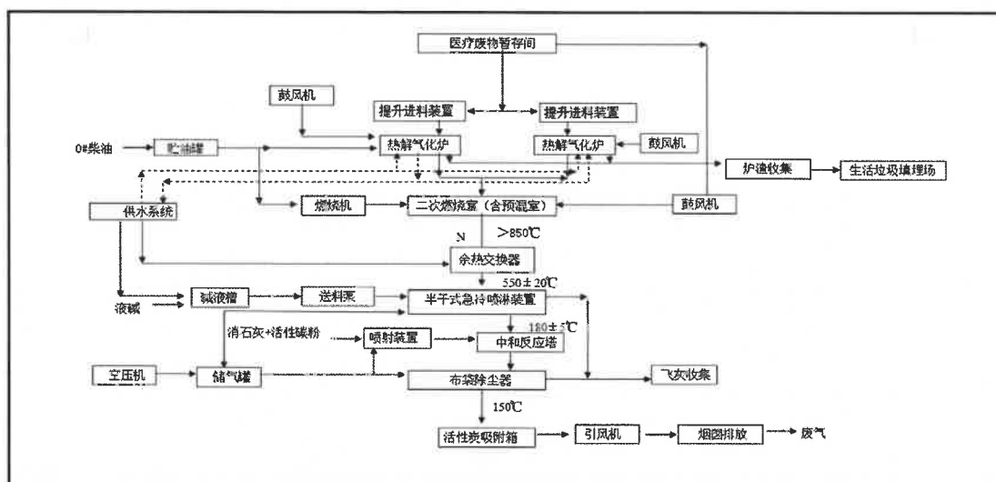
(热解焚烧工艺流程图)
